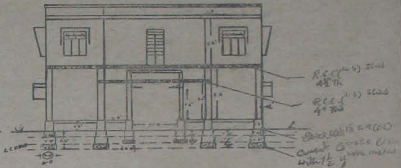
CROSS SECTION ON "A.B."
